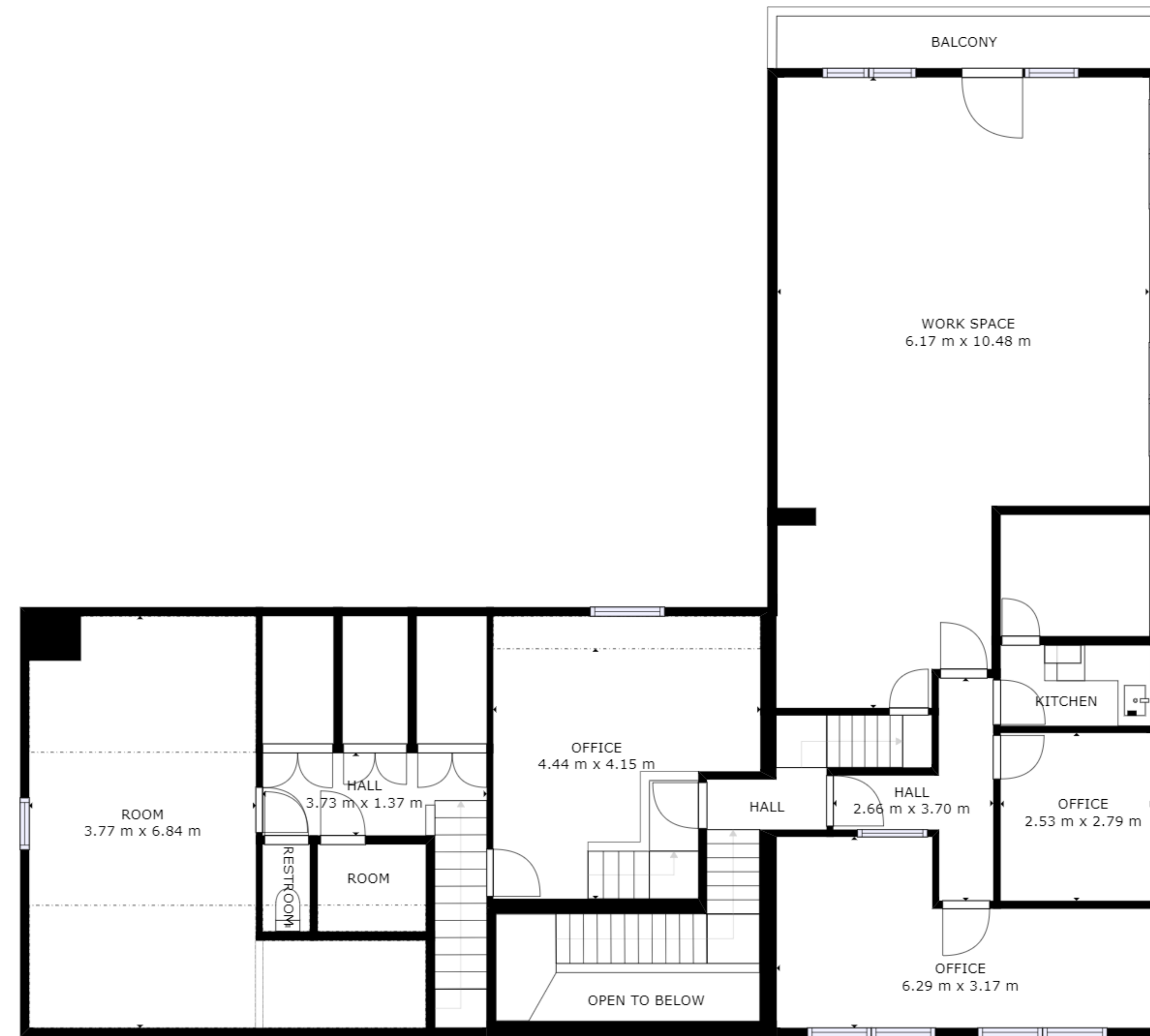
FLOOR 2
