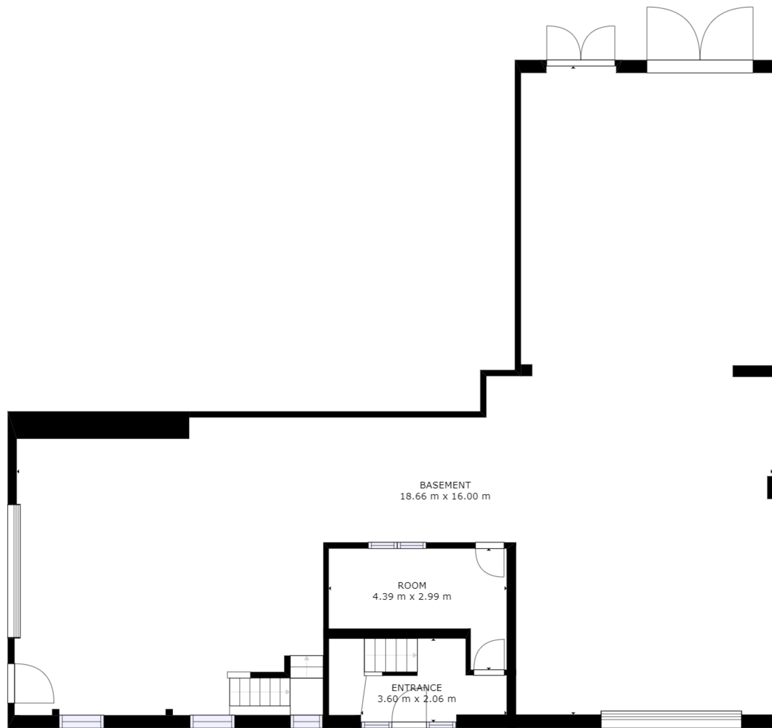
FLOOR 1
