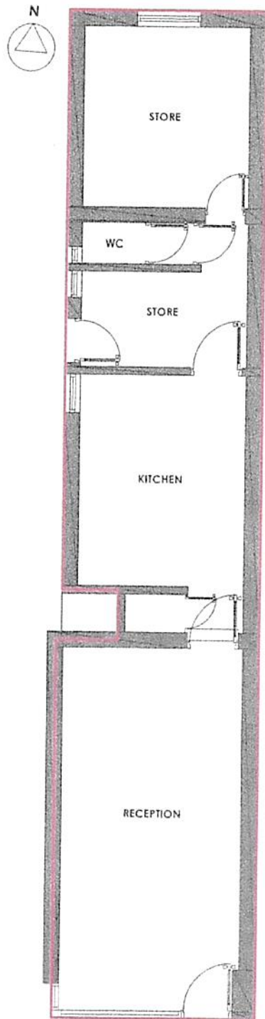
GROUND FLOOR PLAN 1:100&A3
